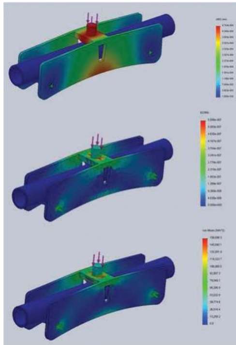
Figure 17. Analysis of presses for bending pipes [5].
