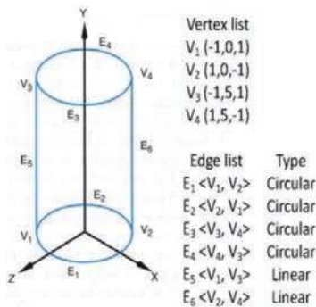
Figure 10. A wireframe model using circular and linear.
