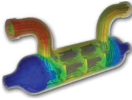
Figure 16. Simulation of the heat exchanger [1].
