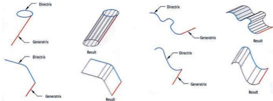
Figure 12. Swept surfaces.
