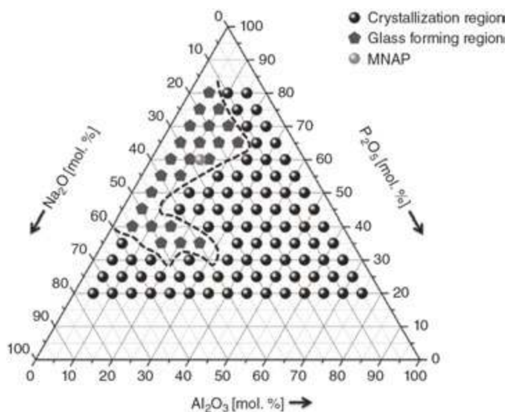
Fig. 6. Ternary phase diagram of \text{Na}_2\text{O}-\text{Al}_2\text{O}_3-\text{P}_2\text{O}_5 system [51],[58].
