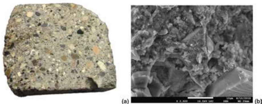
Fig. 4. Cutting plane throughout the block of chemically phosphate bonded refractory material containing large grains of calcined bauxite (a) and electron microscopy (SEM) picture of ceramic body (b).
