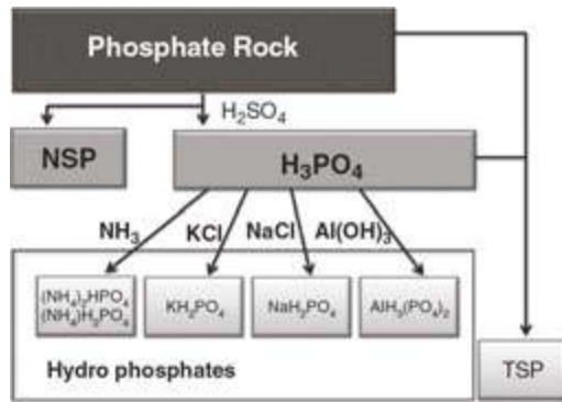
Fig. 1. Flow chart of production of acid phosphates from phosphate ores [1].
