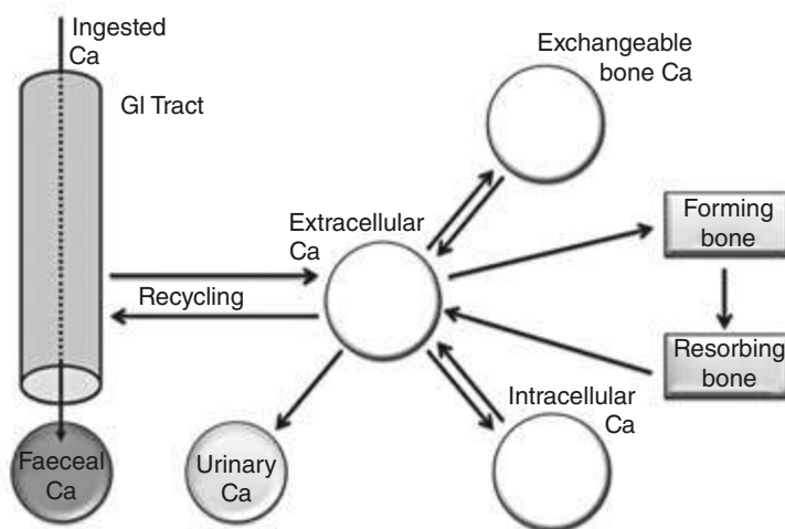
Fig. 15. General scheme of metabolism of calcium [119].
