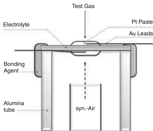
Fig. 11. Schematic picture of the O_2 concentration cell with the electrolyte of Ln_{0.83}Si_{4.5}Al_{1.5}O_{26} where Ln = La, Nd and Sm [86].
