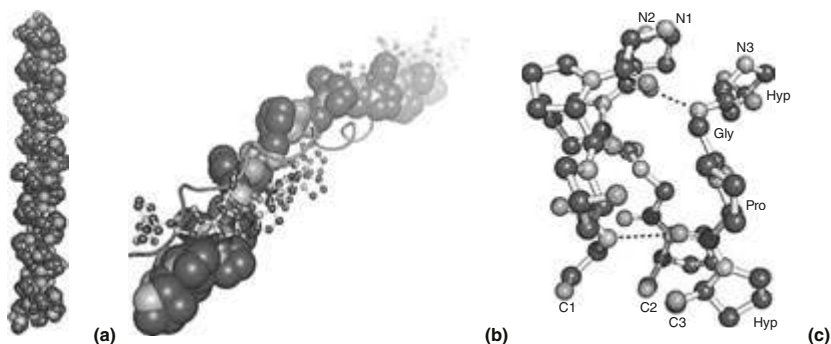
Fig. 18. The triple helix of collagen formed from (\text{PROHYPGLY})_4\text{-(PROHYPALA)}\text{-(PROHYPGLY)}_5 (a), the view down the axis of a (\text{PROPROGLY})_{10} triple helix (b) and the segment of triple helix (c) with hydrogen bonds (—) [129].
