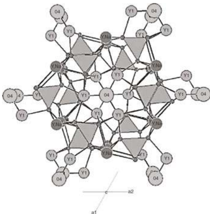
Fig. 7. Crystal structure of oxyapatite \text{NaY}_6(\text{SiO}_4)_6\text{O}_2 (perspective view along the c -axis) where the tetrahedra represents [\text{SiO}_4]^{4-} structural units [76].
